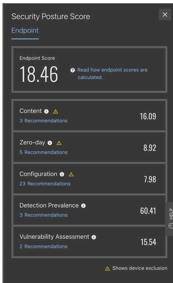
Figure 3. At-a-glance unified and actionable security posture scoring
